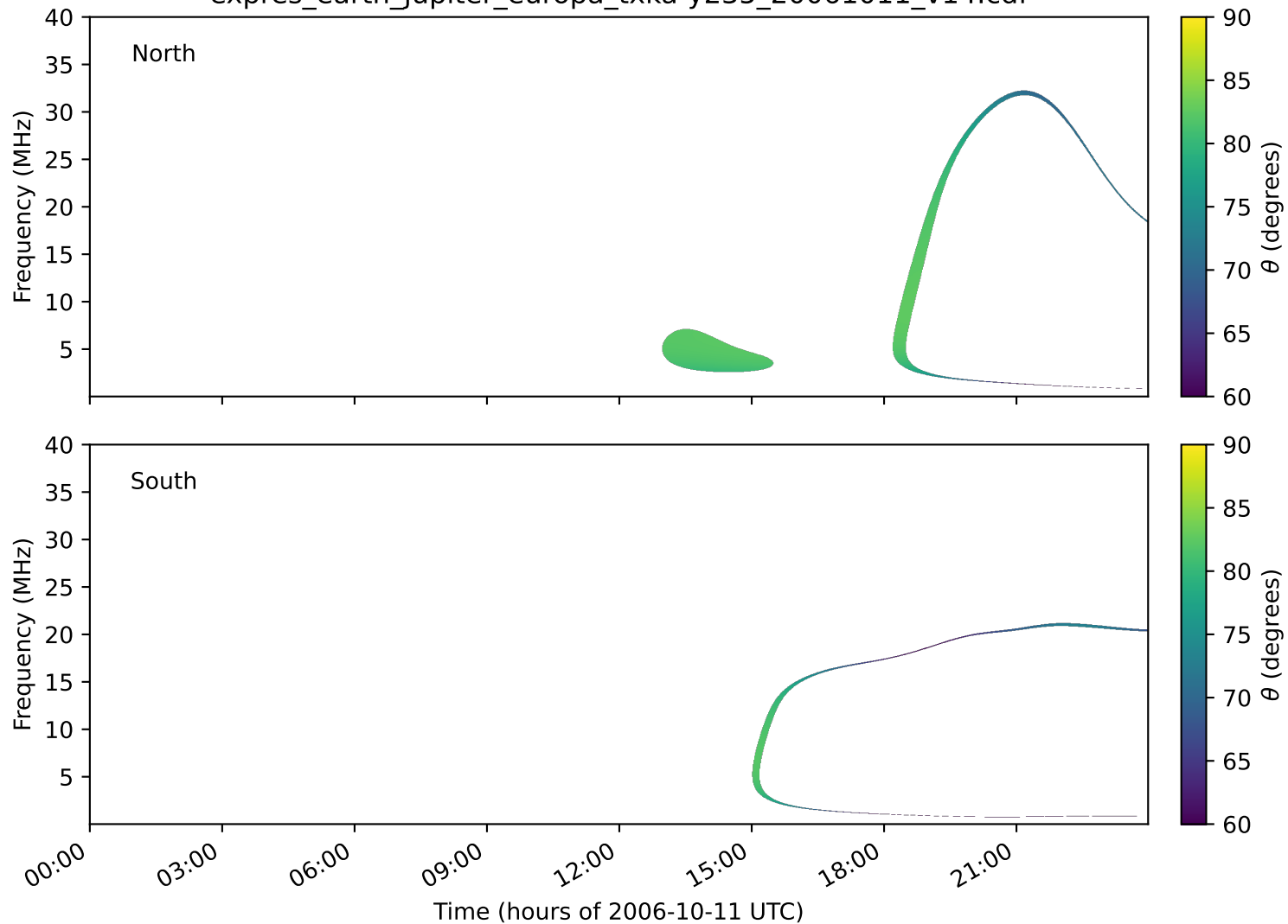
expres_earth_jupiter_europa_txka-y235_20061011_v14.cdf
