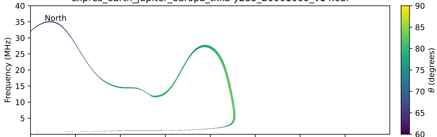
expres_earth_jupiter_europa_txka-y235_20061009_v14.cdf
