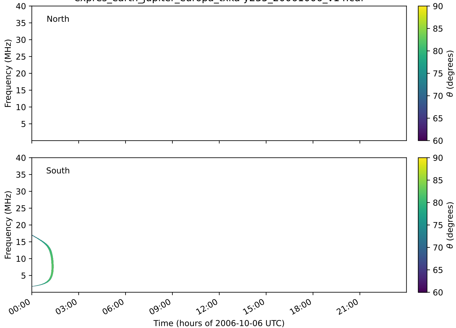
expres_earth_jupiter_europa_txka-y235_20061006_v14.cdf
