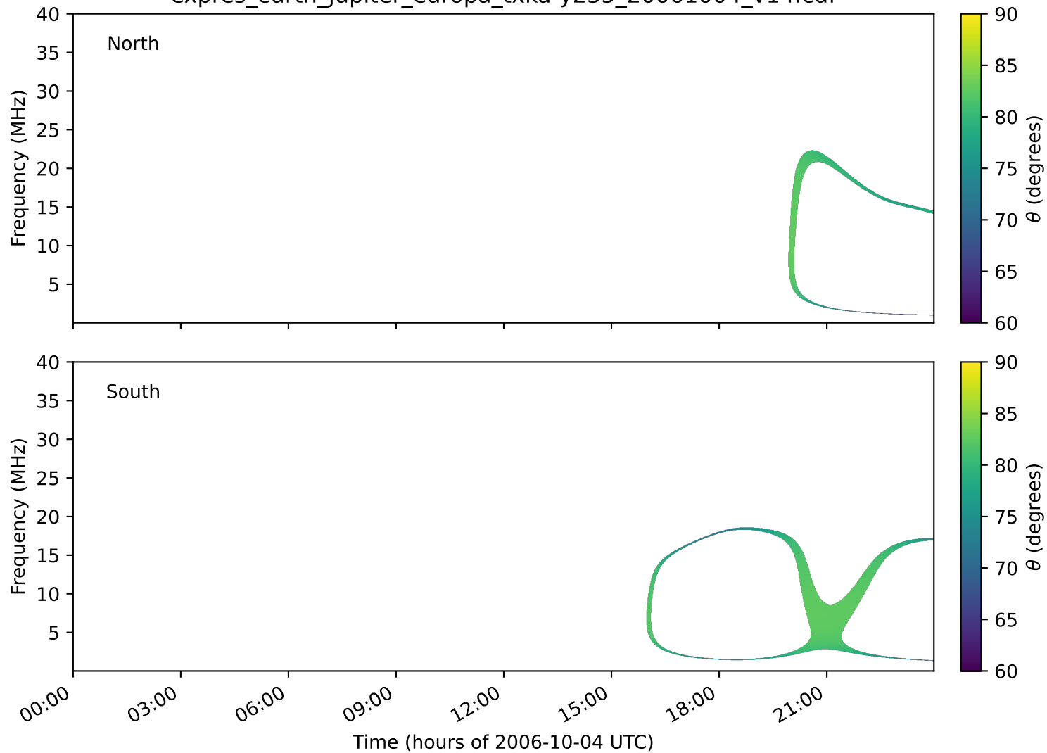
expres_earth_jupiter_europa_txka-y235_20061004_v14.cdf
