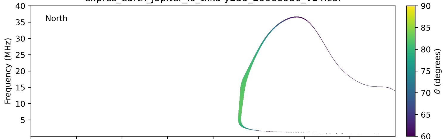
expres_earth_jupiter_io_txka-y235_20060930_v14.cdf
