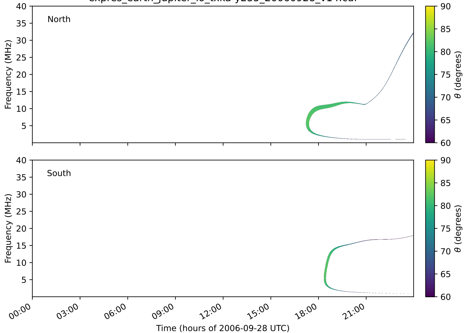
expres_earth_jupiter_io_txka-y235_20060928_v14.cdf
