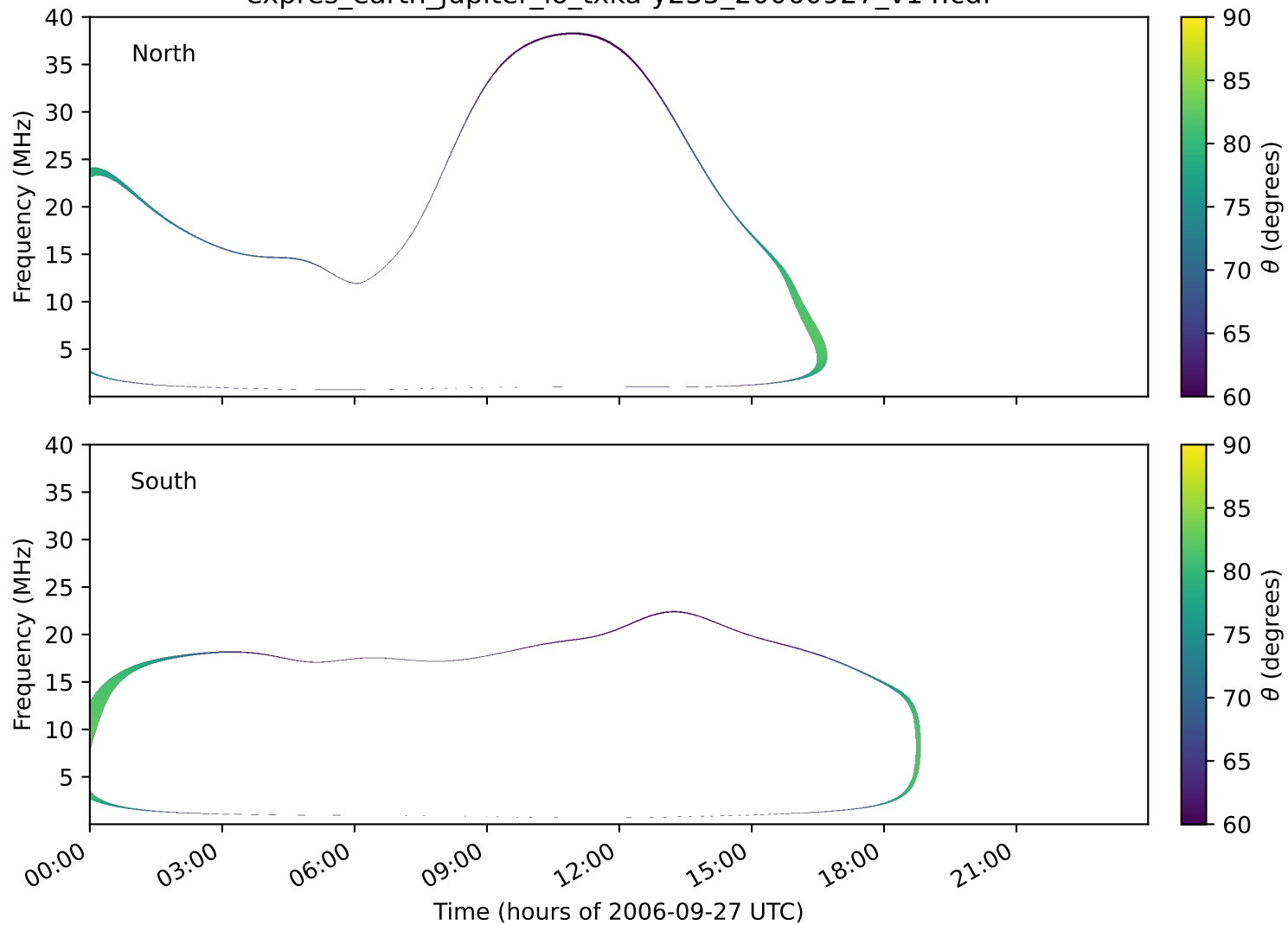
expres_earth_jupiter_io_txka-y235_20060927_v14.cdf
