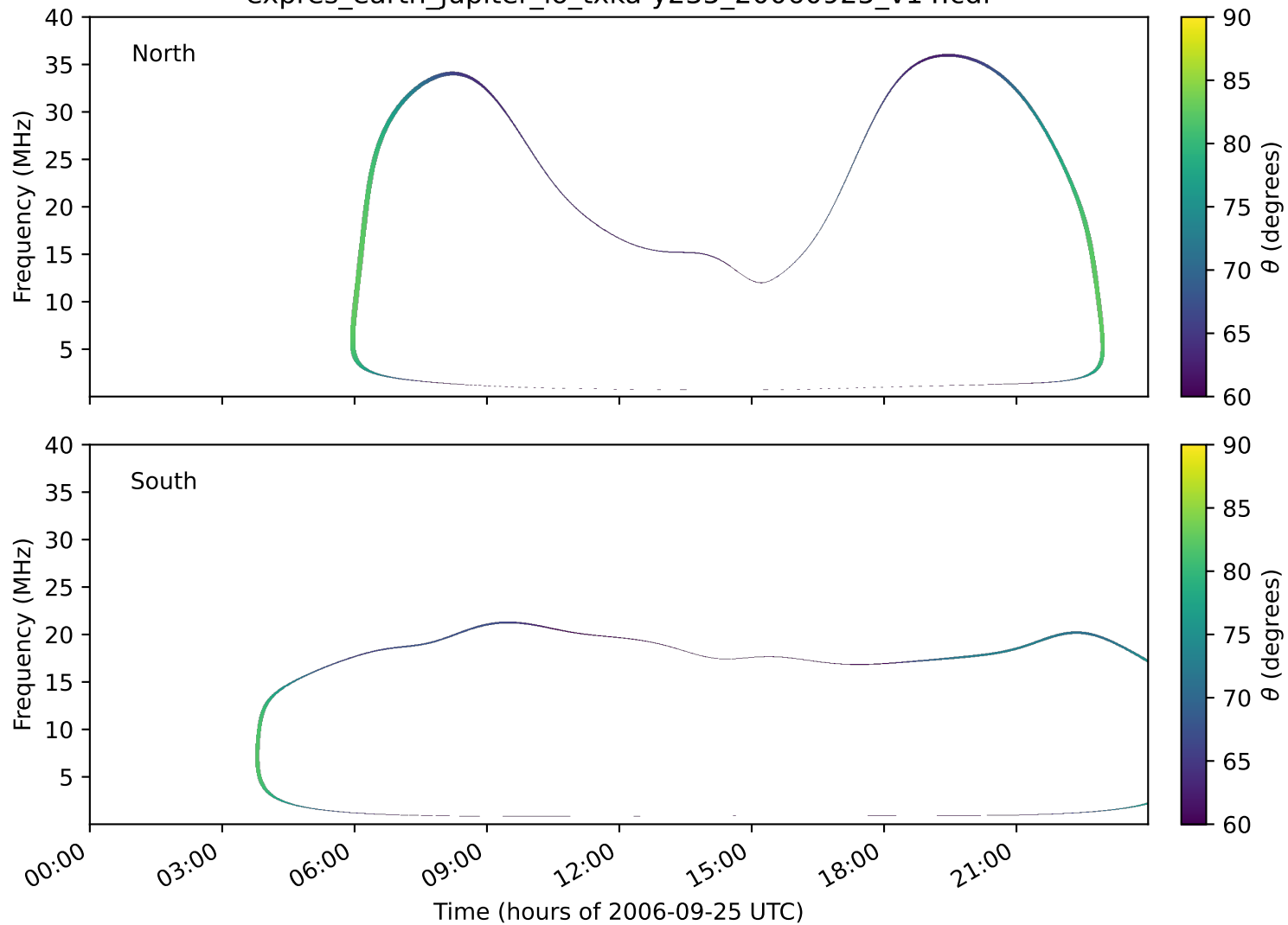
expres_earth_jupiter_io_txka-y235_20060925_v14.cdf
