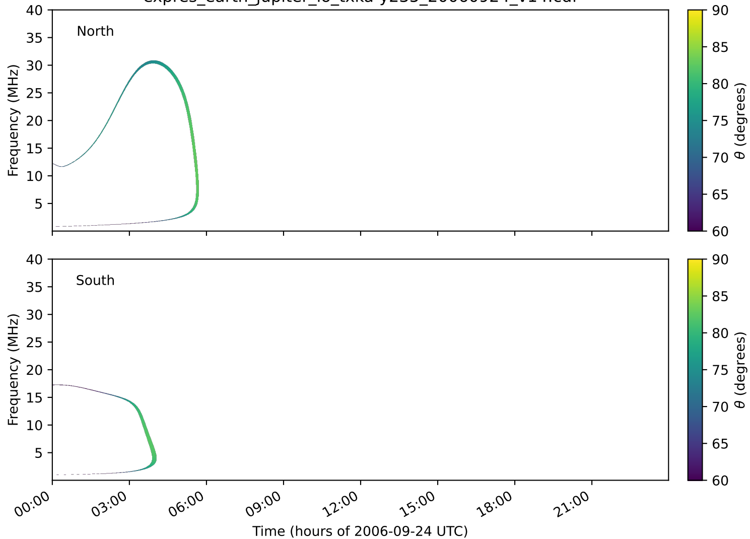
expres_earth_jupiter_io_txka-y235_20060924_v14.cdf
