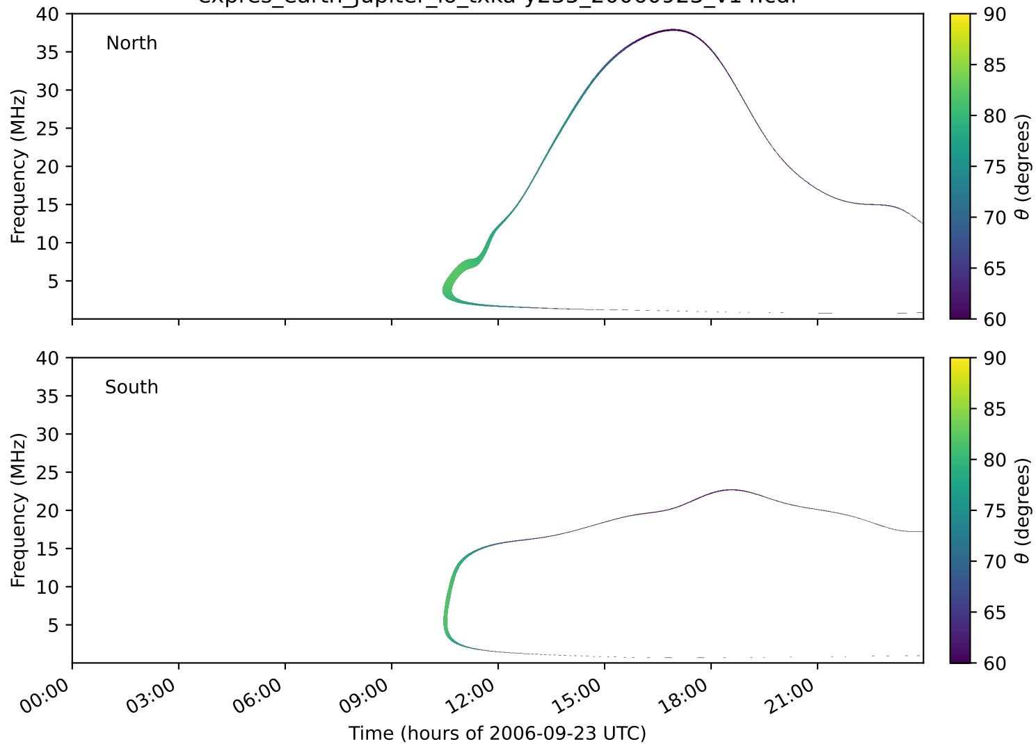
expres_earth_jupiter_io_txka-y235_20060923_v14.cdf
