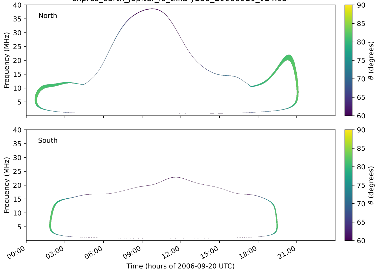
expres_earth_jupiter_io_txka-y235_20060920_v14.cdf
