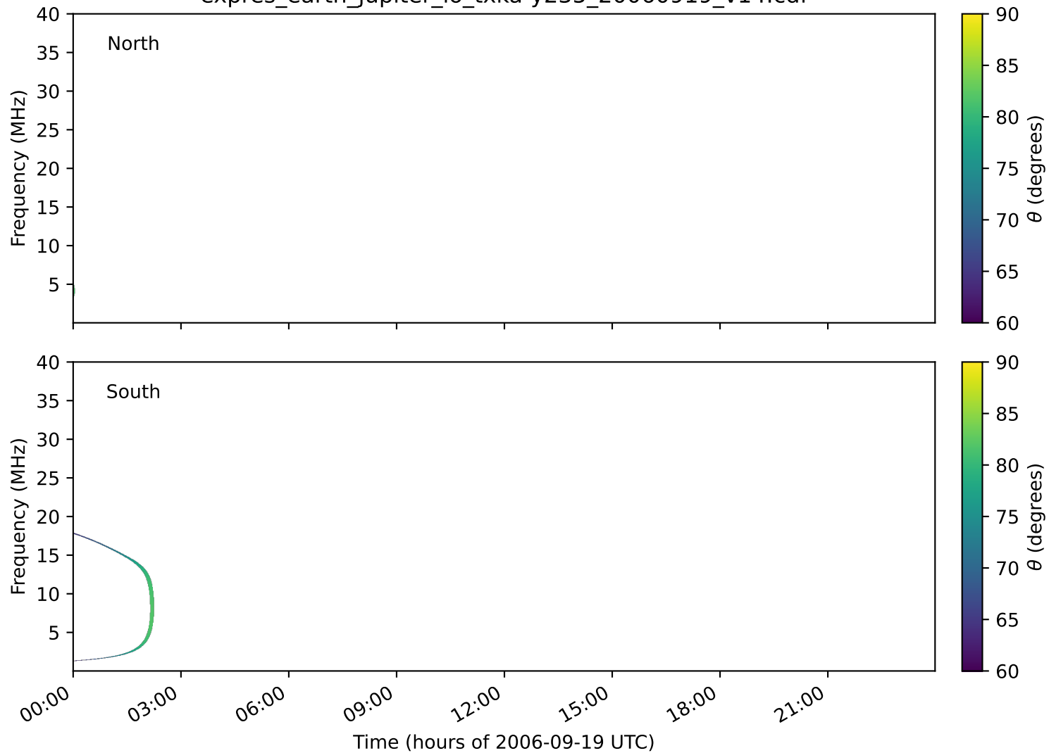
expres_earth_jupiter_io_txka-y235_20060919_v14.cdf
