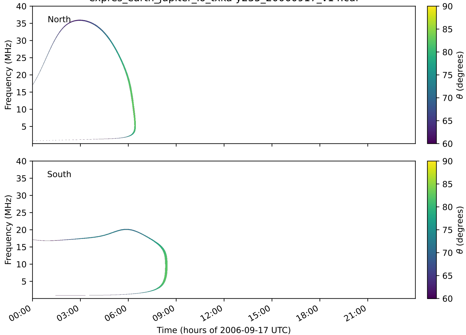
expres_earth_jupiter_io_txka-y235_20060917_v14.cdf
