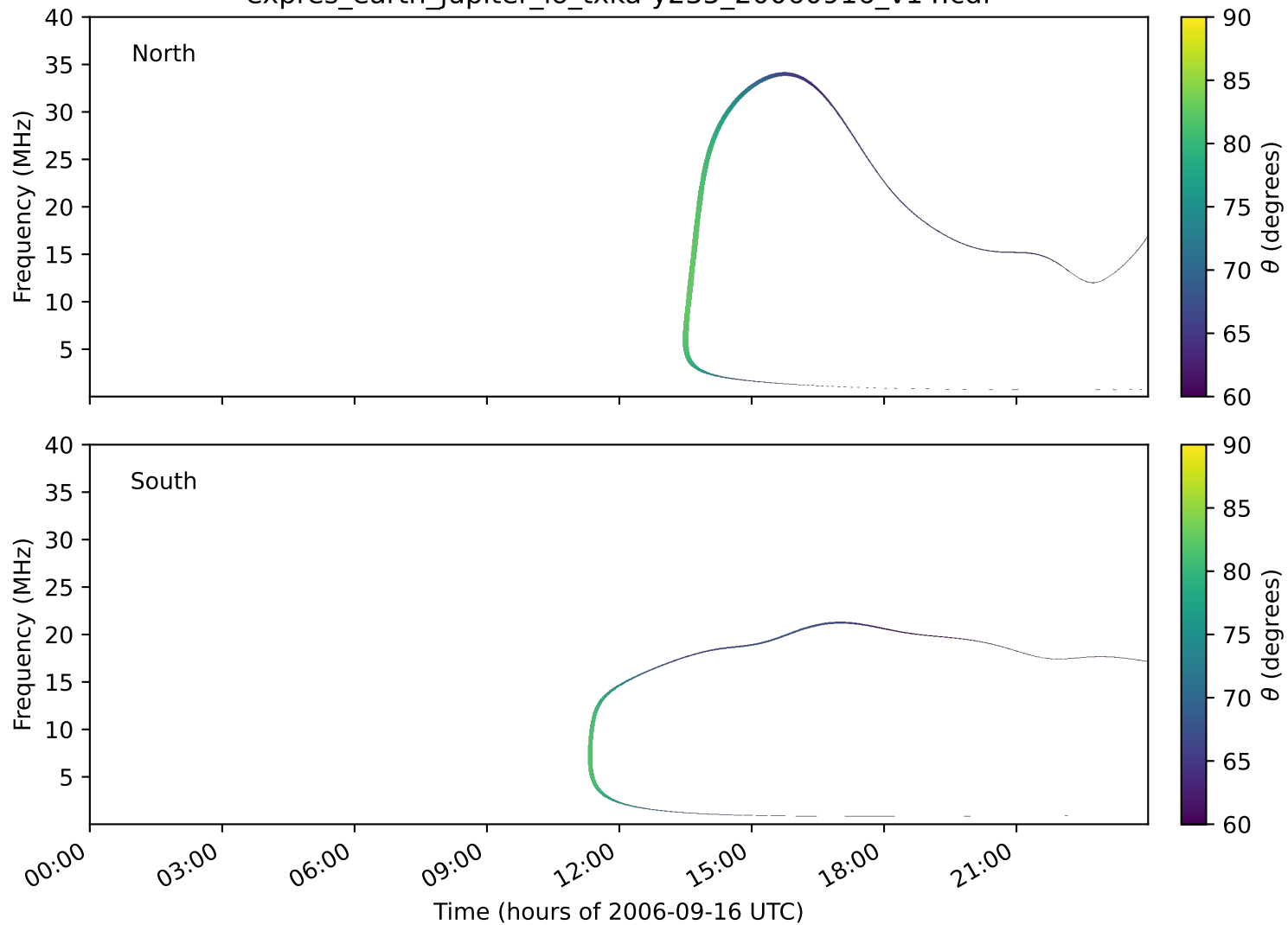
expres_earth_jupiter_io_txka-y235_20060916_v14.cdf
