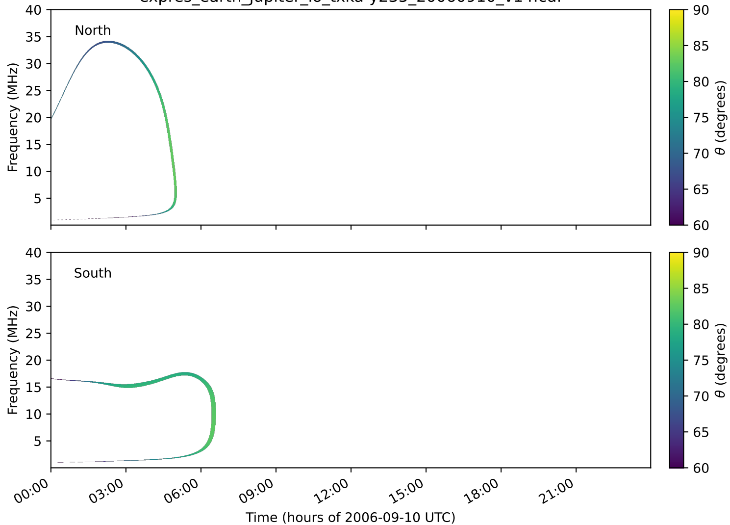
expres_earth_jupiter_io_txka-y235_20060910_v14.cdf
