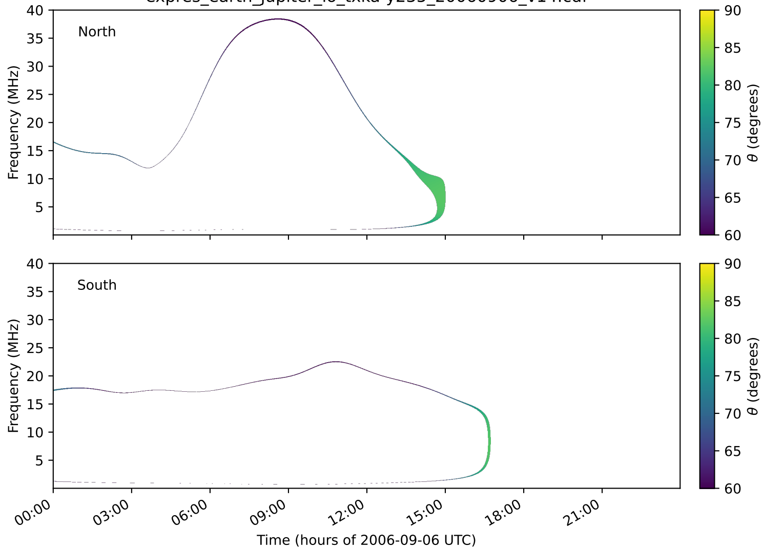
expres_earth_jupiter_io_txka-y235_20060906_v14.cdf
