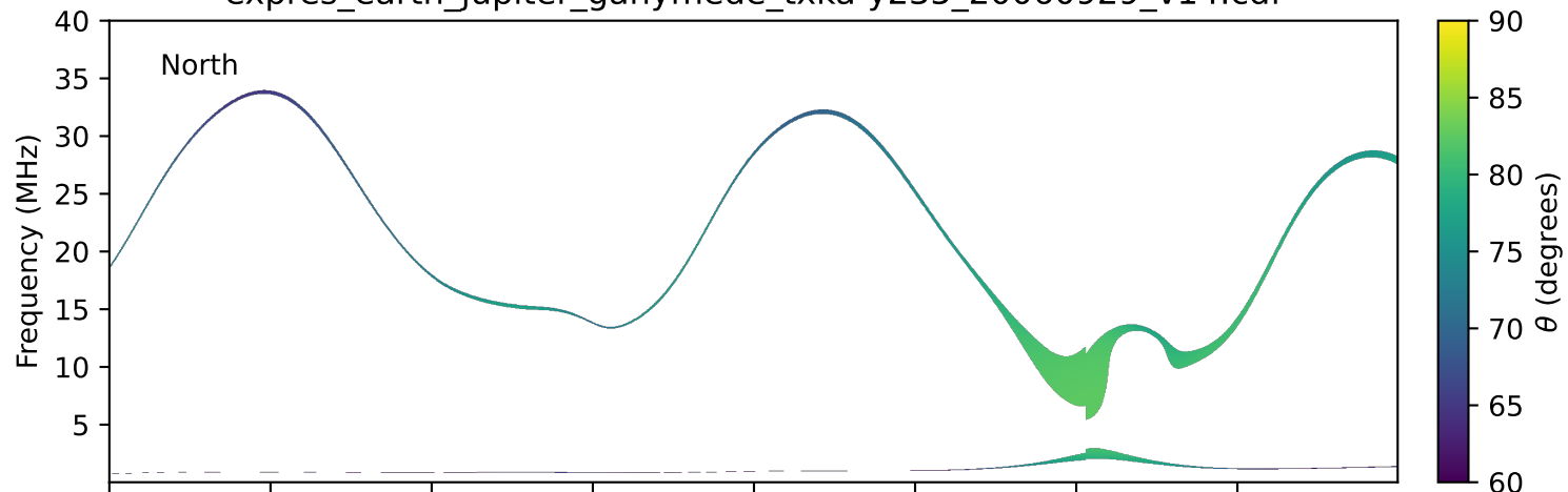
expres_earth_jupiter_ganymede_txka-y235_20060929_v14.cdf
