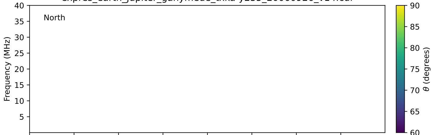
expres_earth_jupiter_ganymede_txka-y235_20060926_v14.cdf
