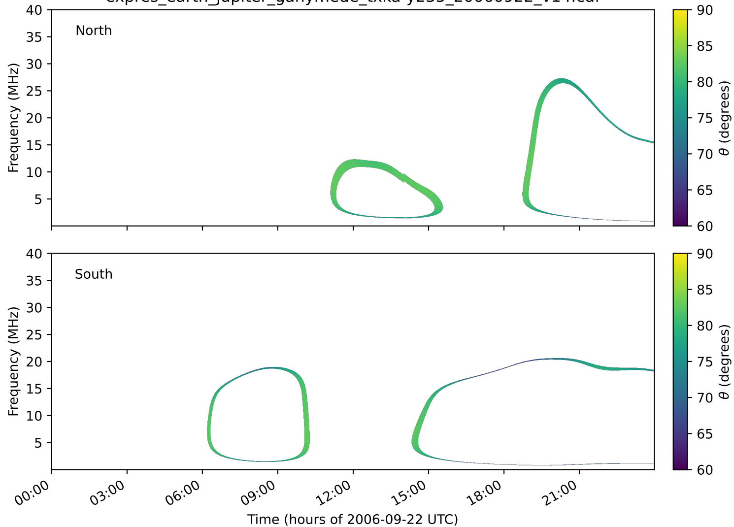
expres_earth_jupiter_ganymede_txka-y235_20060922_v14.cdf
