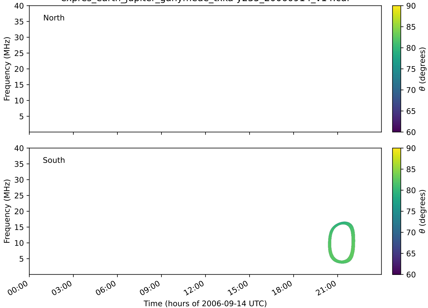
expres_earth_jupiter_ganymede_txka-y235_20060914_v14.cdf
