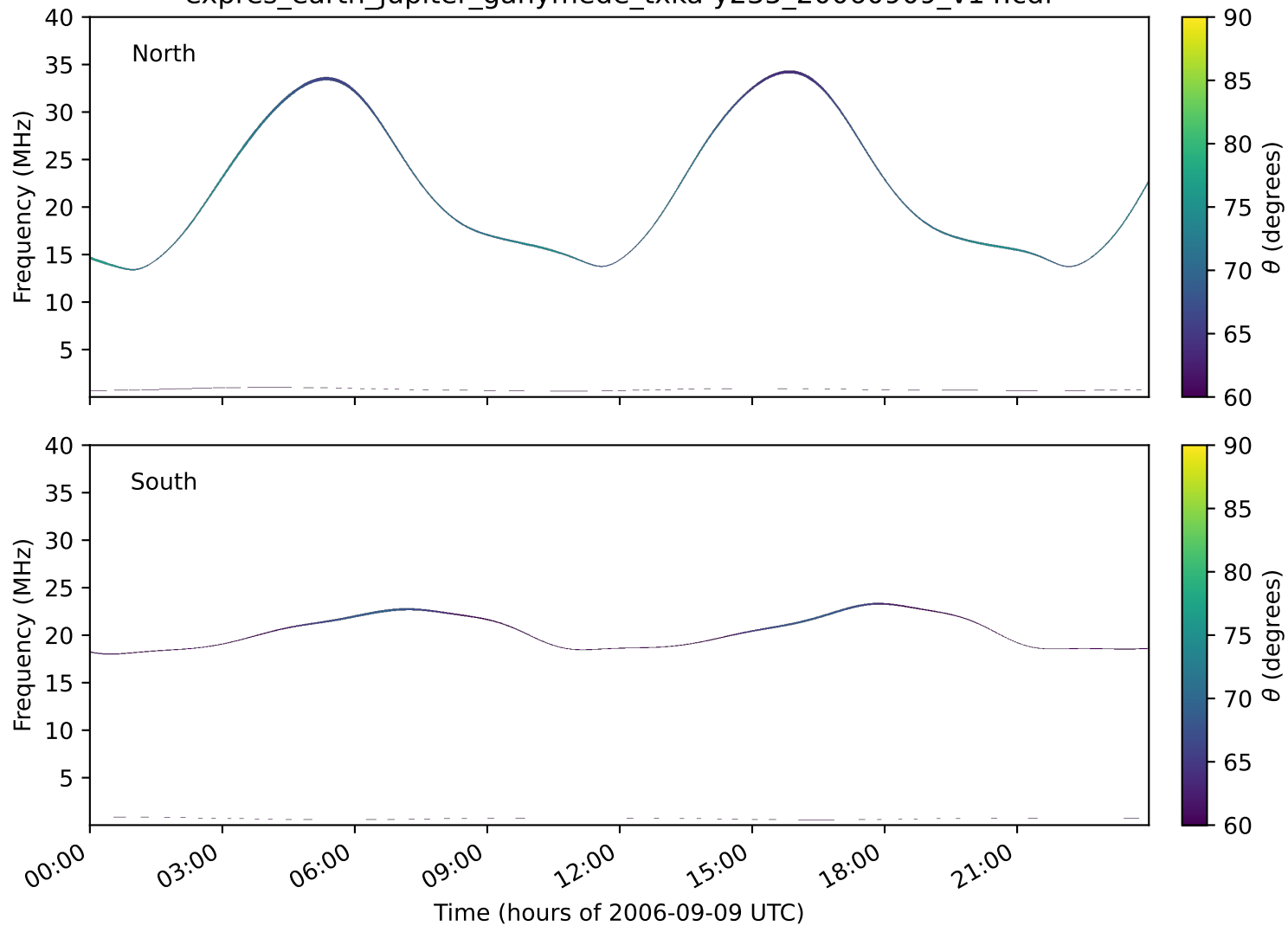
expres_earth_jupiter_ganymede_txka-y235_20060909_v14.cdf
