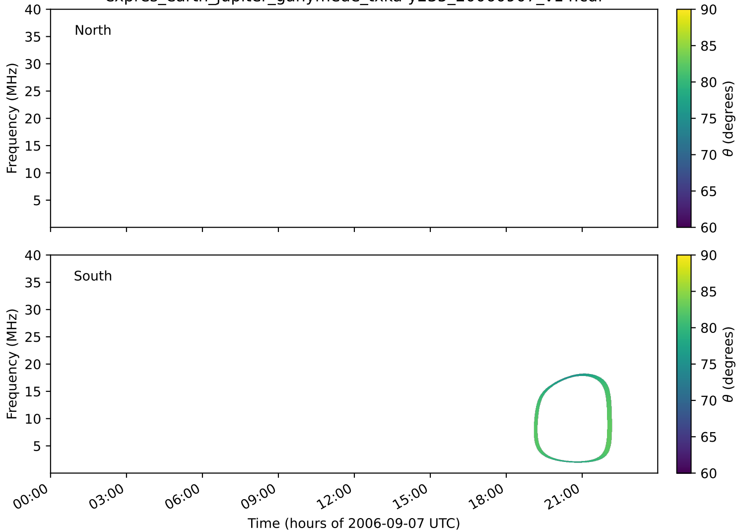
expres_earth_jupiter_ganymede_txka-y235_20060907_v14.cdf
