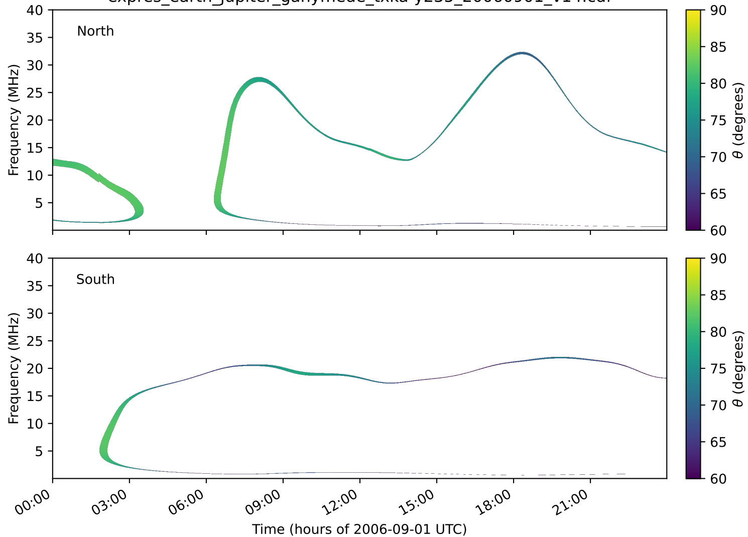
expres_earth_jupiter_ganymede_txka-y235_20060901_v14.cdf
