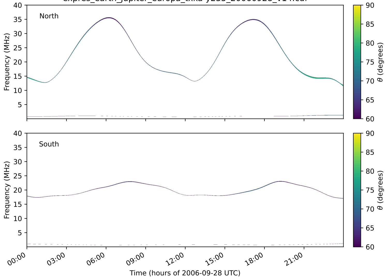
expres_earth_jupiter_europa_txka-y235_20060928_v14.cdf
