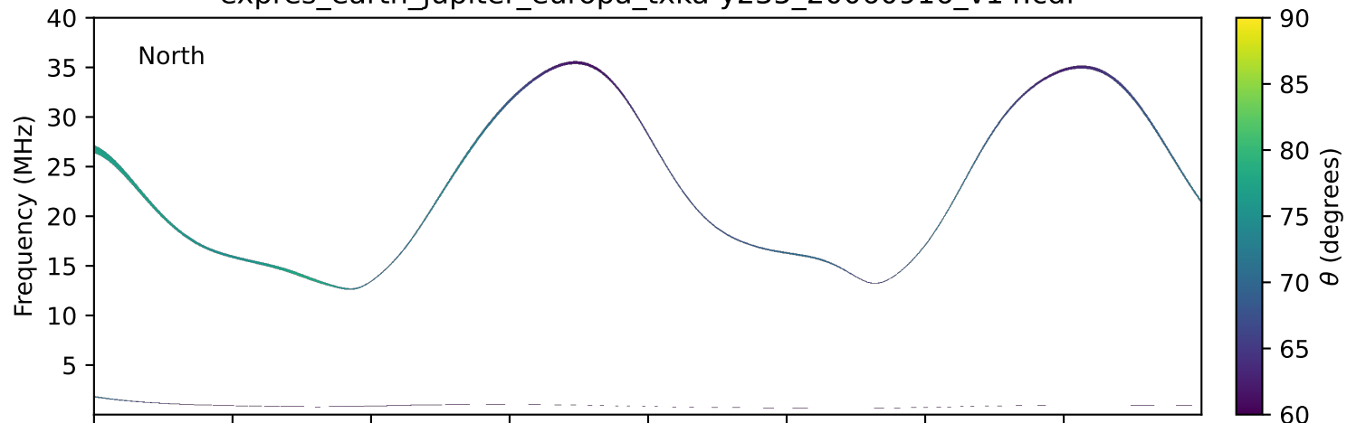
expres_earth_jupiter_europa_txka-y235_20060916_v14.cdf
