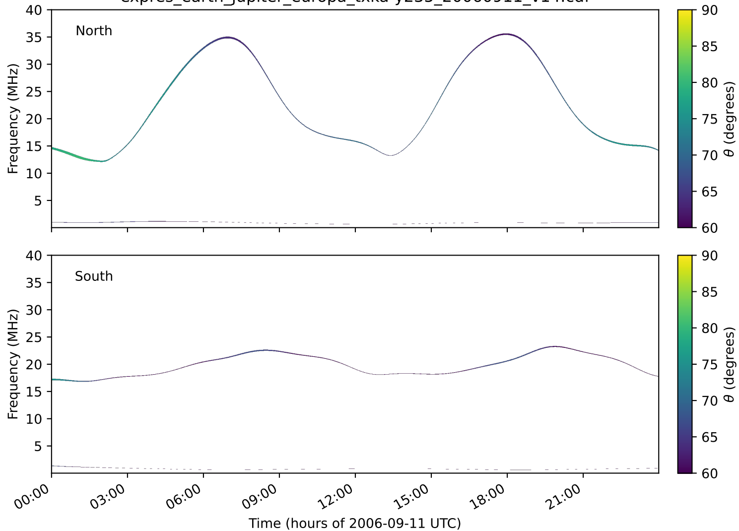
expres_earth_jupiter_europa_txka-y235_20060911_v14.cdf
