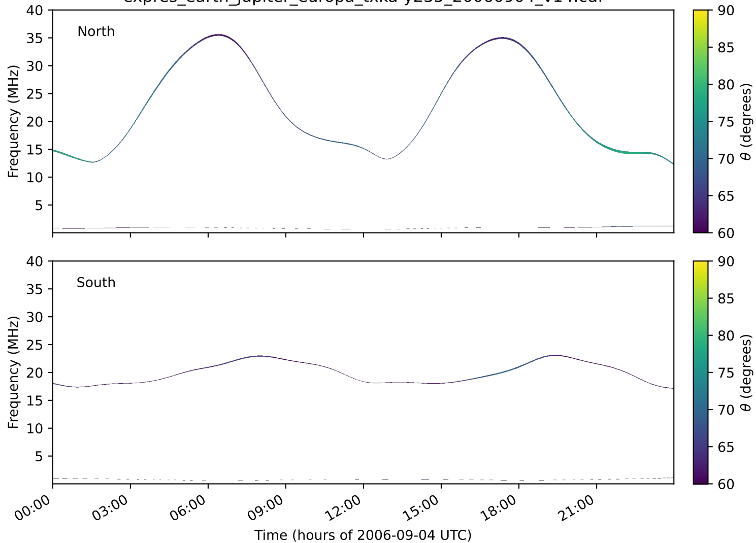
expres_earth_jupiter_europa_txka-y235_20060904_v14.cdf
