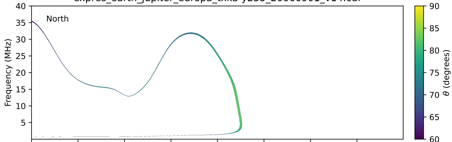
expres_earth_jupiter_europa_txka-y235_20060901_v14.cdf
