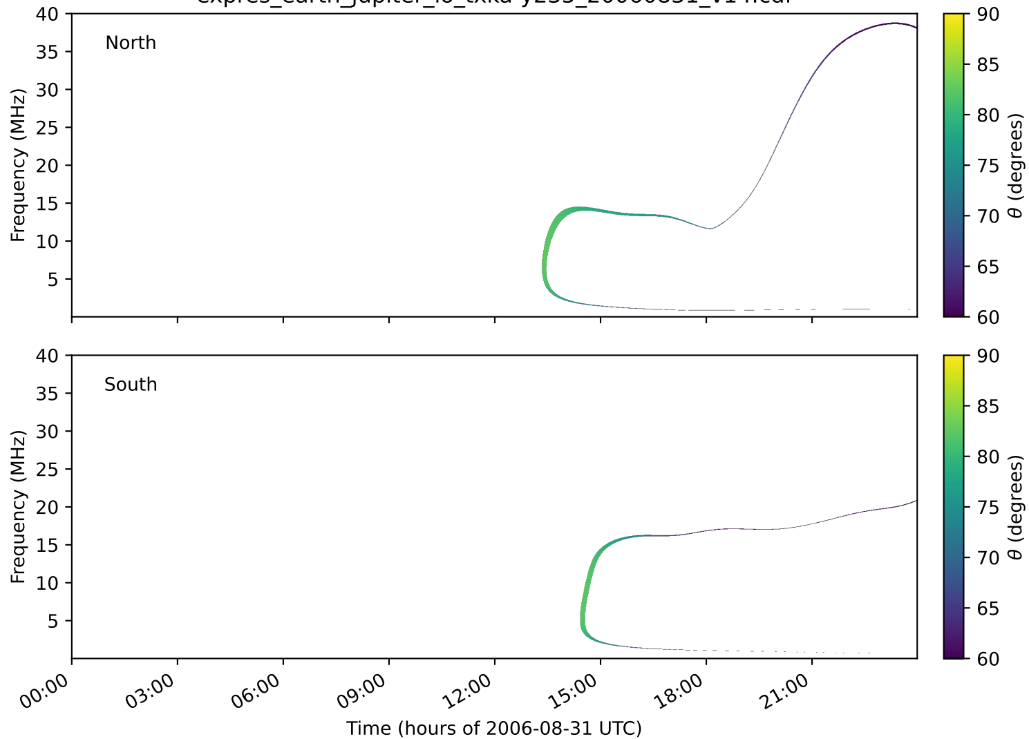
expres_earth_jupiter_io_txka-y235_20060831_v14.cdf
