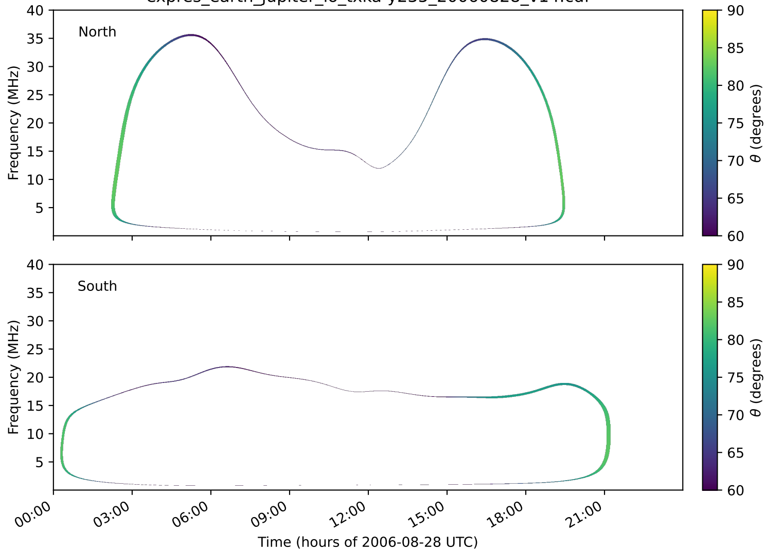
expres_earth_jupiter_io_txka-y235_20060828_v14.cdf
