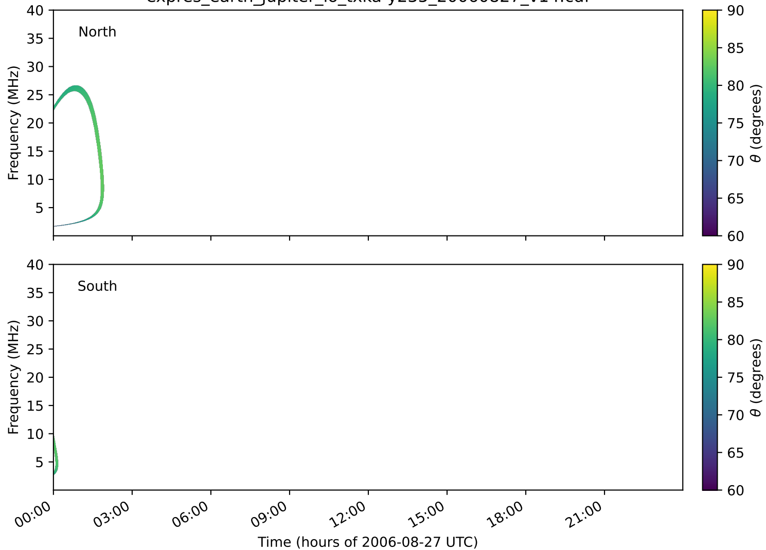
expres_earth_jupiter_io_txka-y235_20060827_v14.cdf
