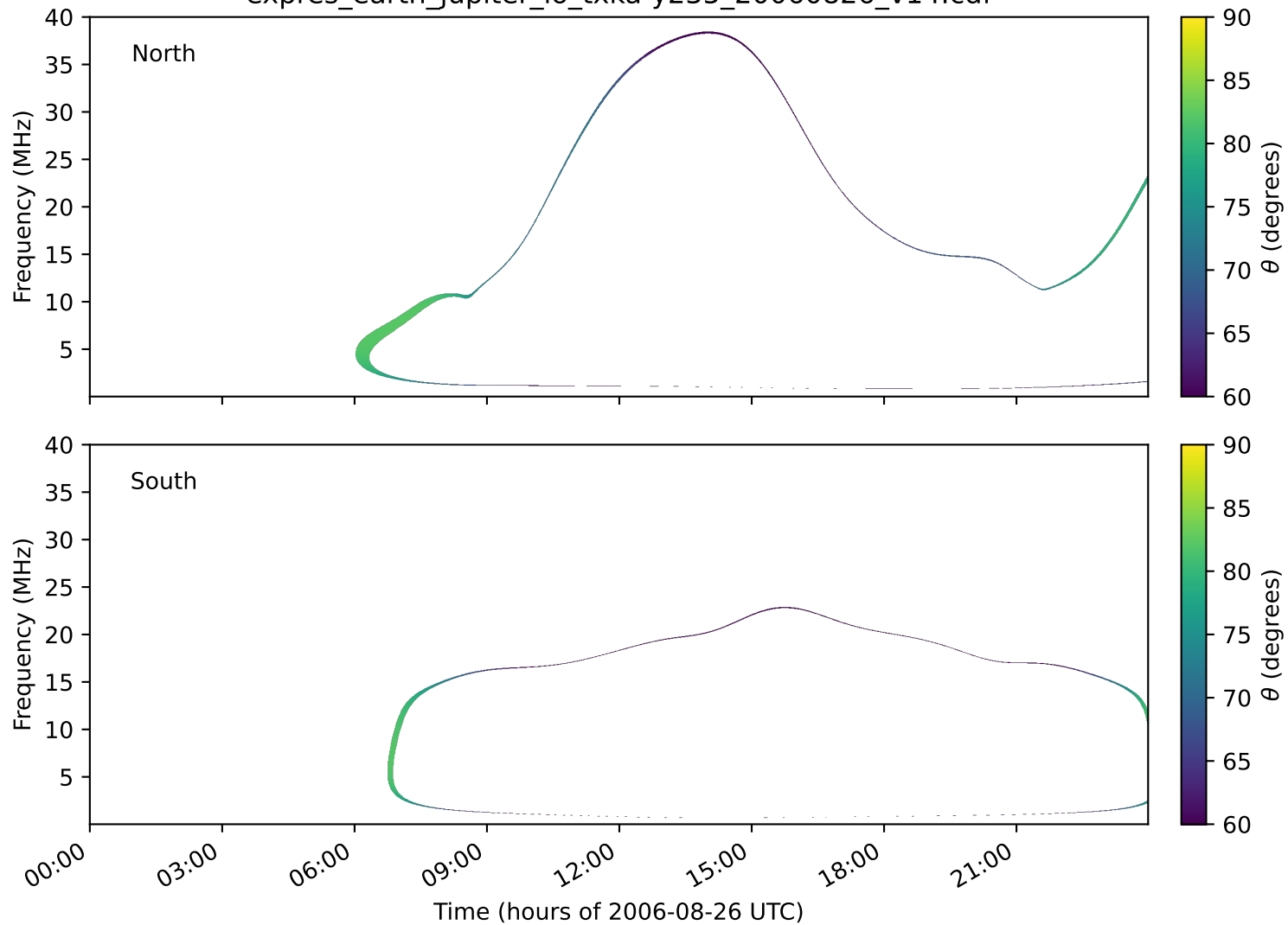
expres_earth_jupiter_io_txka-y235_20060826_v14.cdf
