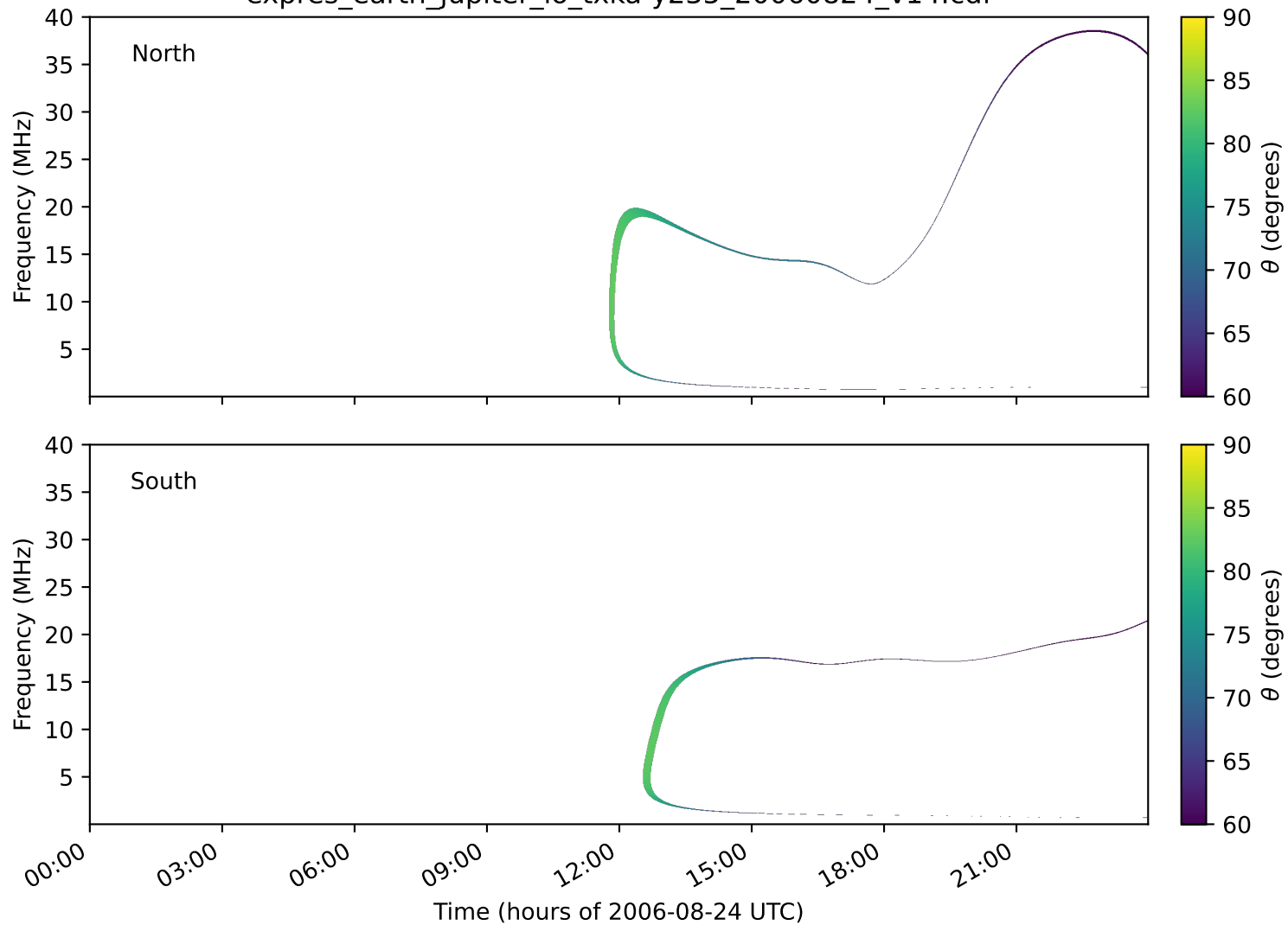
expres_earth_jupiter_io_txka-y235_20060824_v14.cdf
