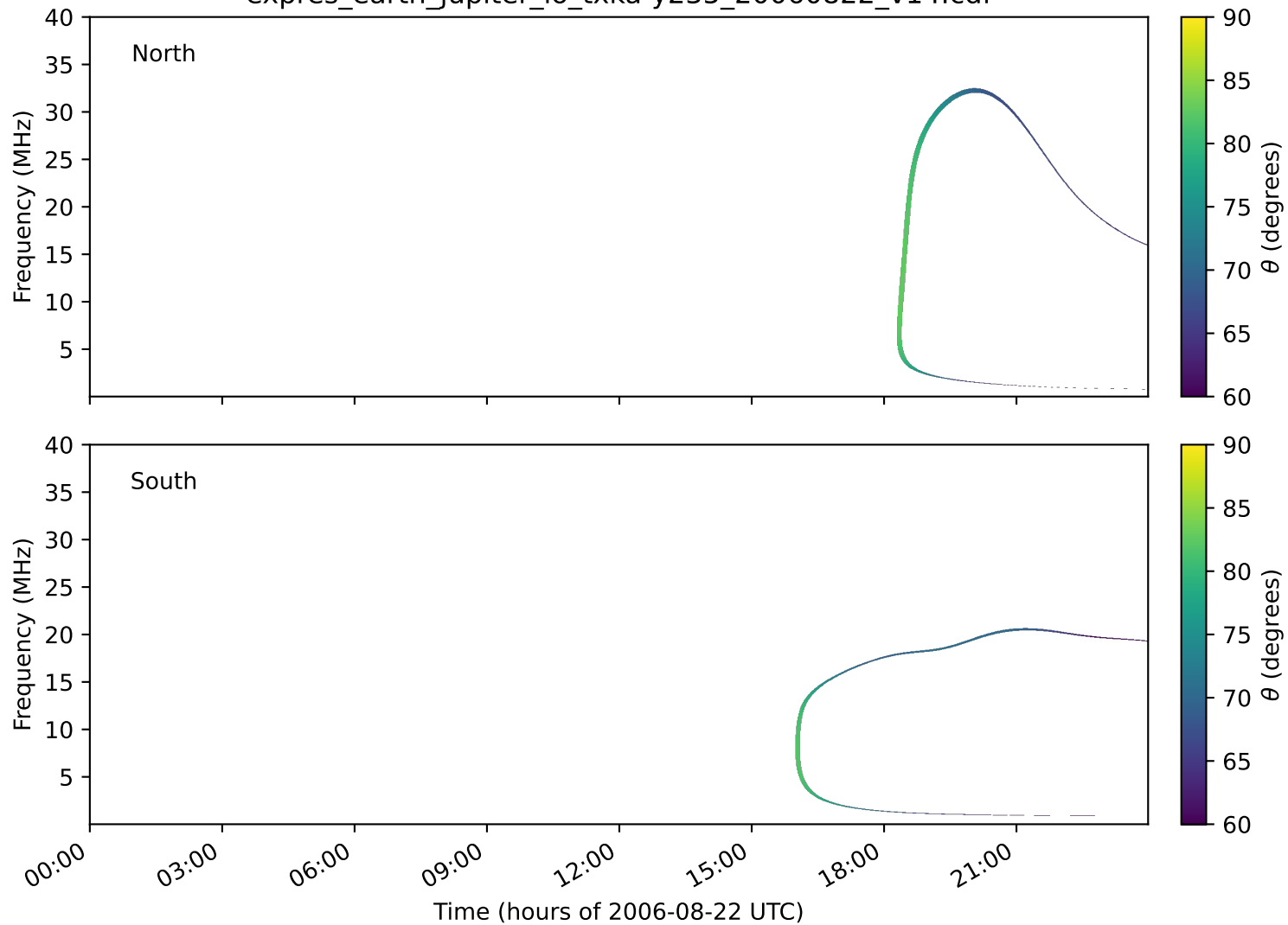
expres_earth_jupiter_io_txka-y235_20060822_v14.cdf
