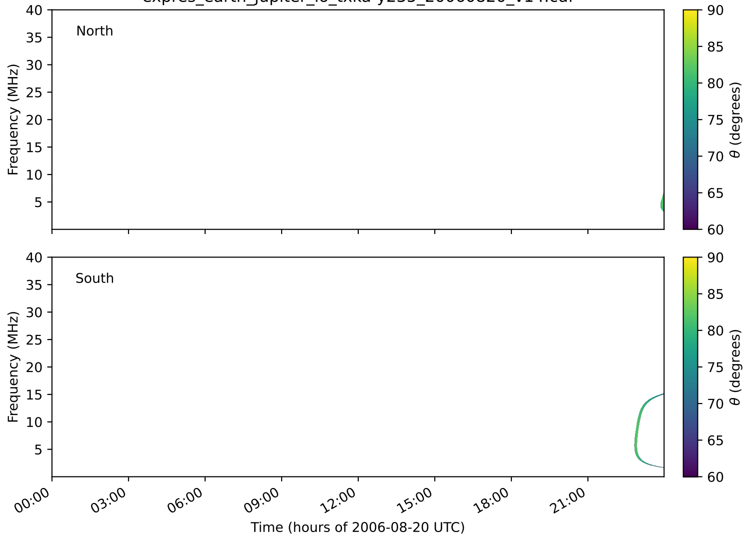
expres_earth_jupiter_io_txka-y235_20060820_v14.cdf
