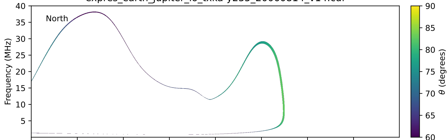
expres_earth_jupiter_io_txka-y235_20060814_v14.cdf
