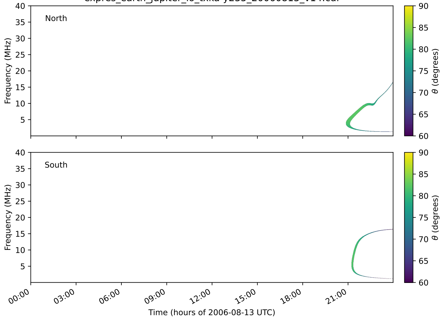
expres_earth_jupiter_io_txka-y235_20060813_v14.cdf
