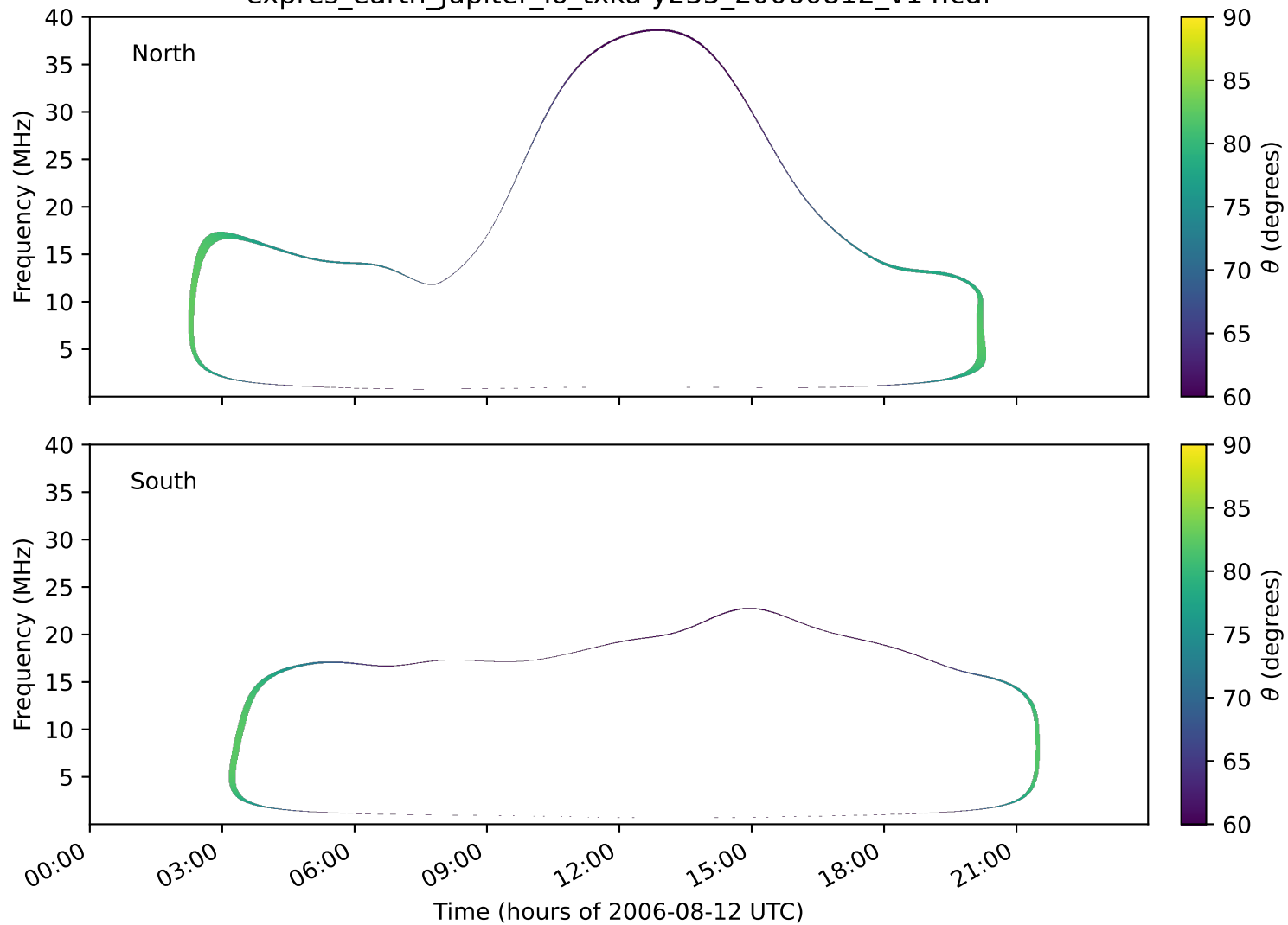
expres_earth_jupiter_io_txka-y235_20060812_v14.cdf
