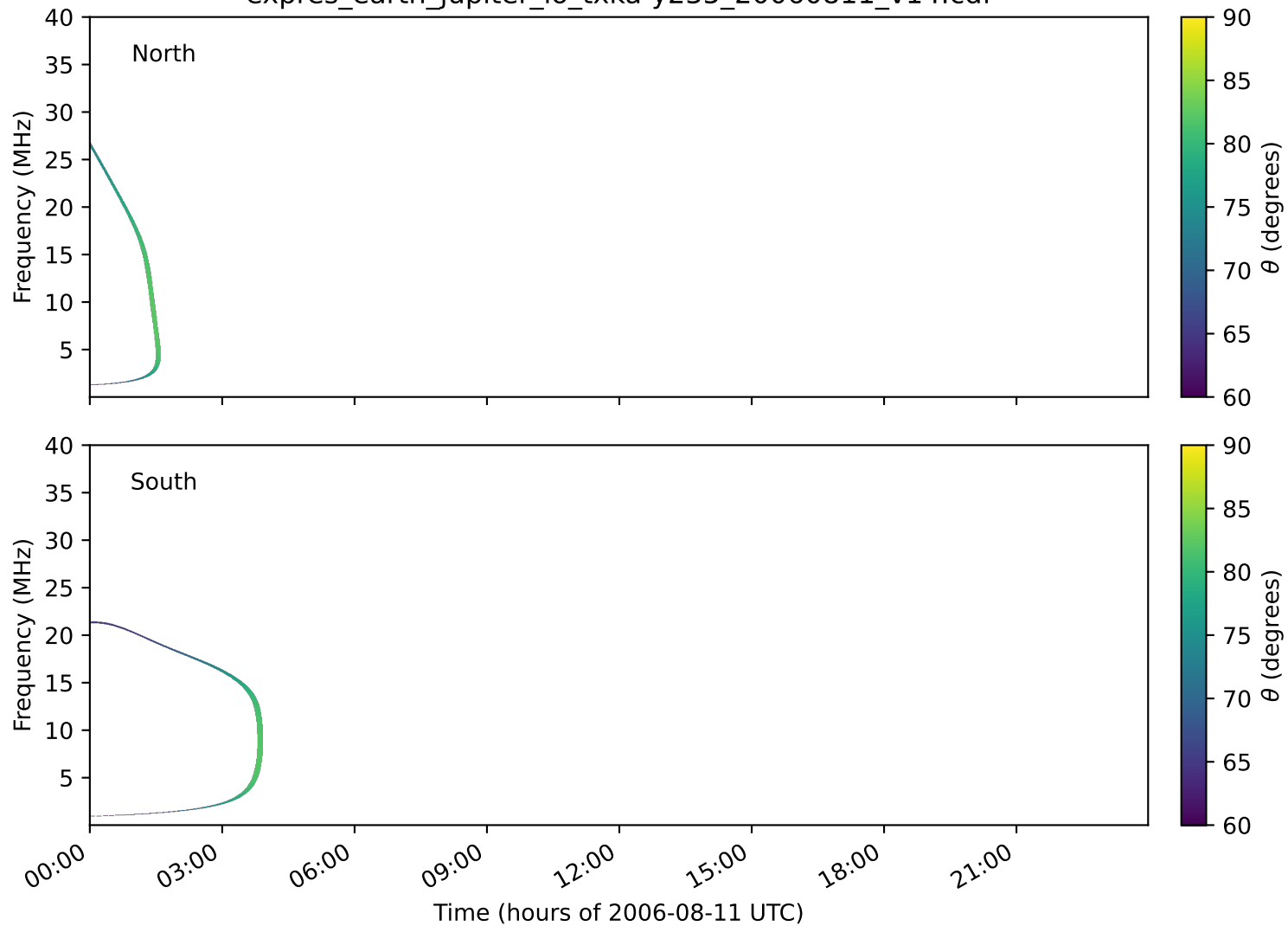
expres_earth_jupiter_io_txka-y235_20060811_v14.cdf
