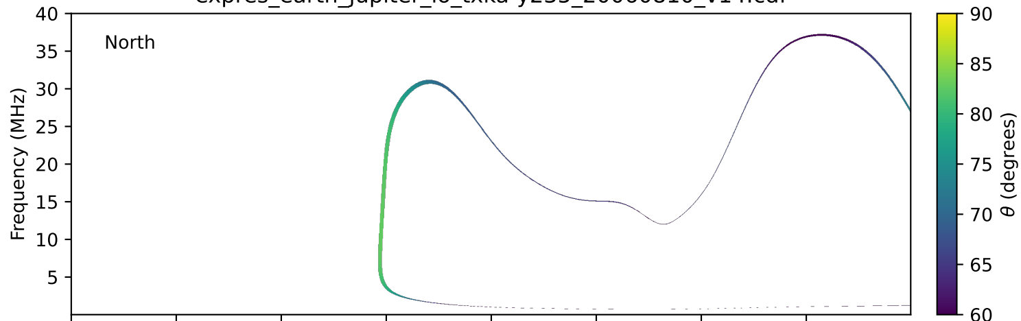
expres_earth_jupiter_io_txka-y235_20060810_v14.cdf
