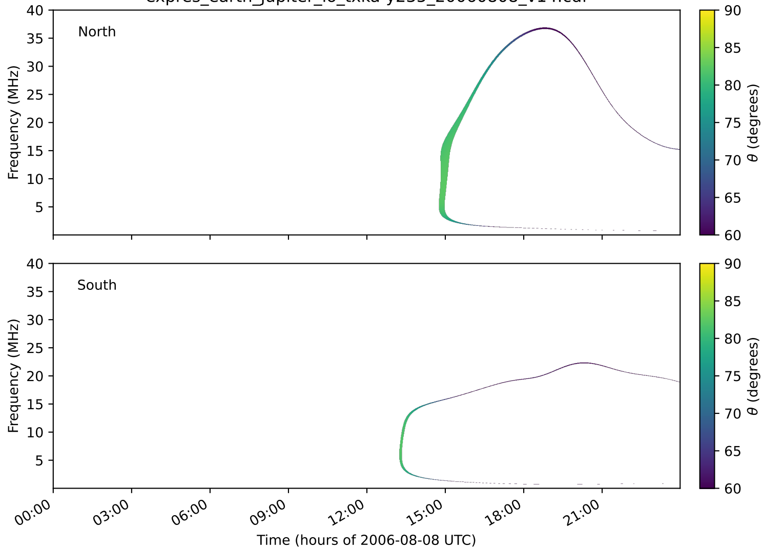
expres_earth_jupiter_io_txka-y235_20060808_v14.cdf
