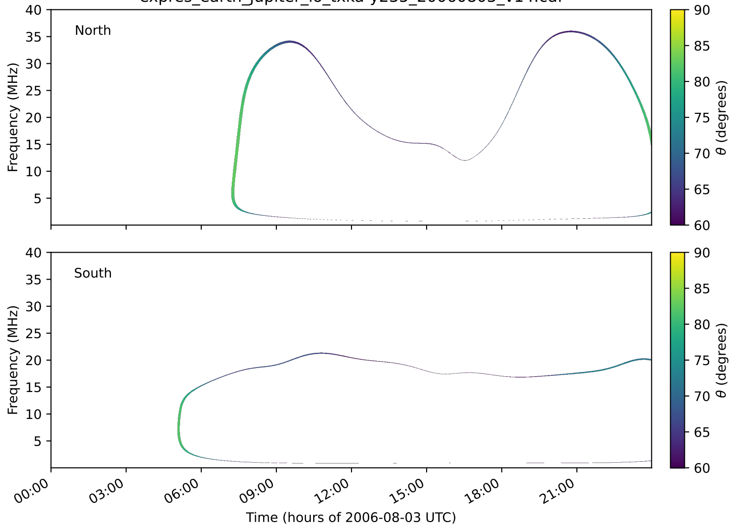
expres_earth_jupiter_io_txka-y235_20060803_v14.cdf
