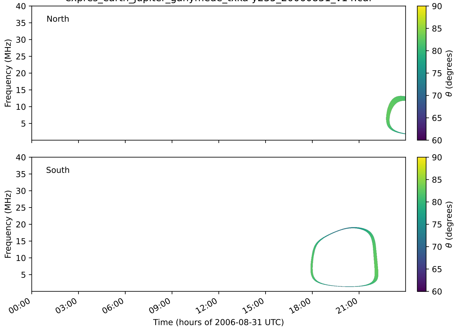
expres_earth_jupiter_ganymede_txka-y235_20060831_v14.cdf
