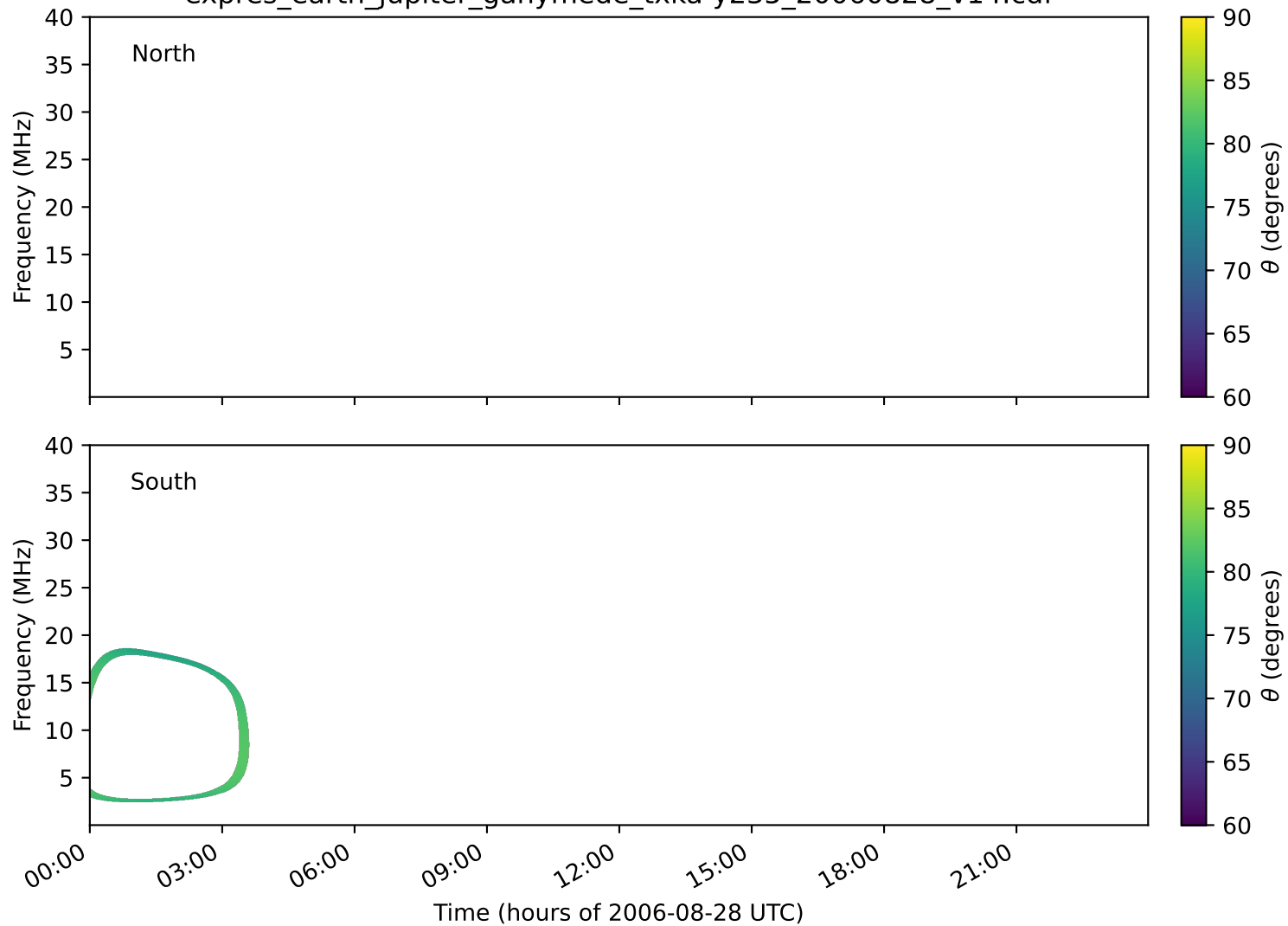
expres_earth_jupiter_ganymede_txka-y235_20060828_v14.cdf
