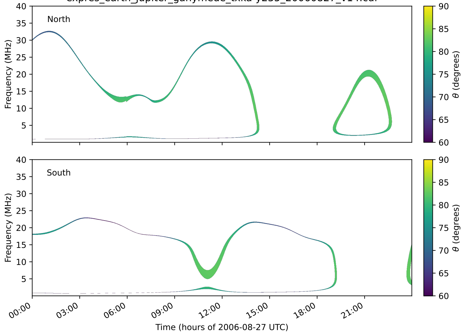
expres_earth_jupiter_ganymede_txka-y235_20060827_v14.cdf
