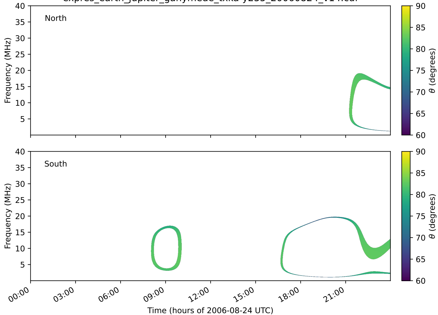
expres_earth_jupiter_ganymede_txka-y235_20060824_v14.cdf
