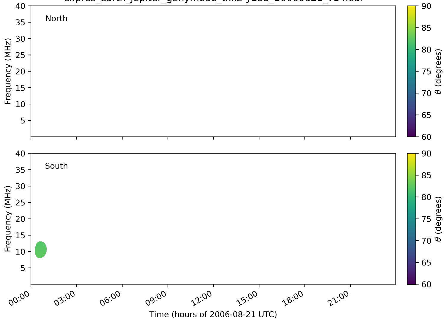
expres_earth_jupiter_ganymede_txka-y235_20060821_v14.cdf
