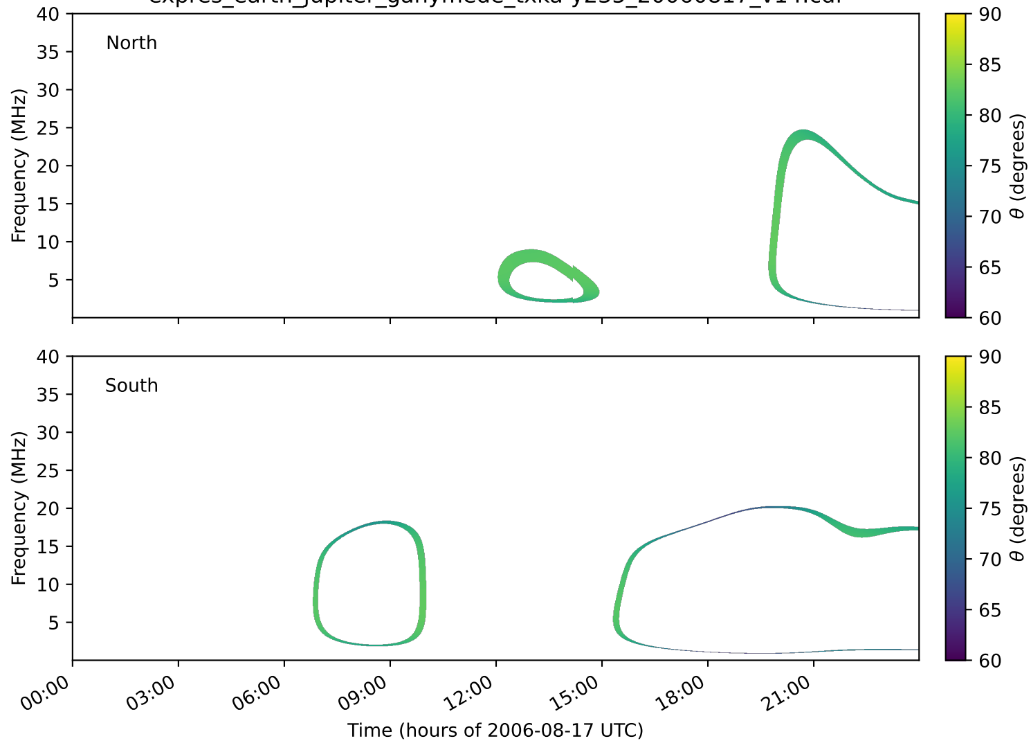
expres_earth_jupiter_ganymede_txka-y235_20060817_v14.cdf
