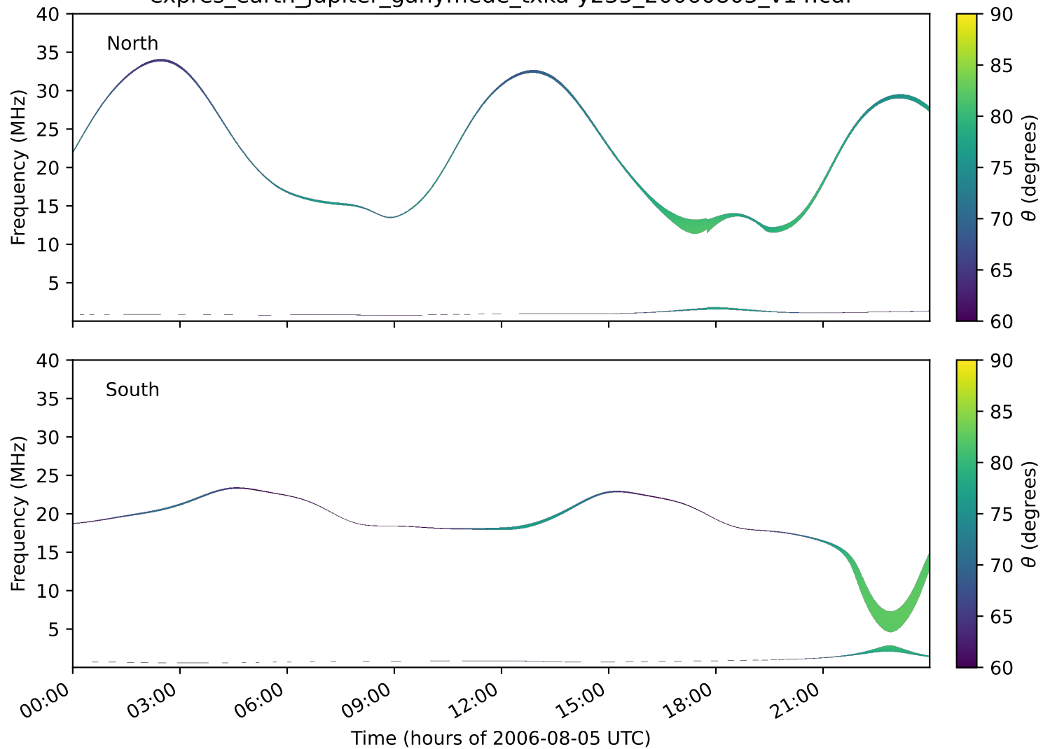
expres_earth_jupiter_ganymede_txka-y235_20060805_v14.cdf
