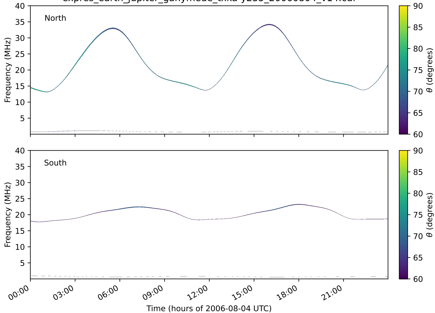
expres_earth_jupiter_ganymede_txka-y235_20060804_v14.cdf
